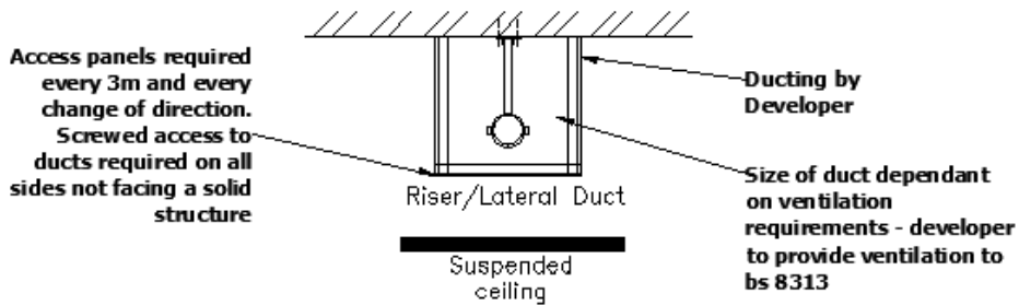
Figure 33 – Ventilation (front elevation)
