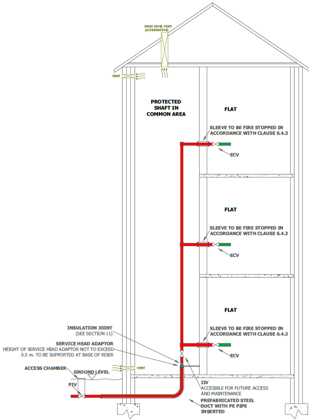
Figure 25 – Internal screwed riser passing through a protective shaft on an outside wall ventilated direct to outside air at the top and bottom of the riser. Meter locations back on to the riser
