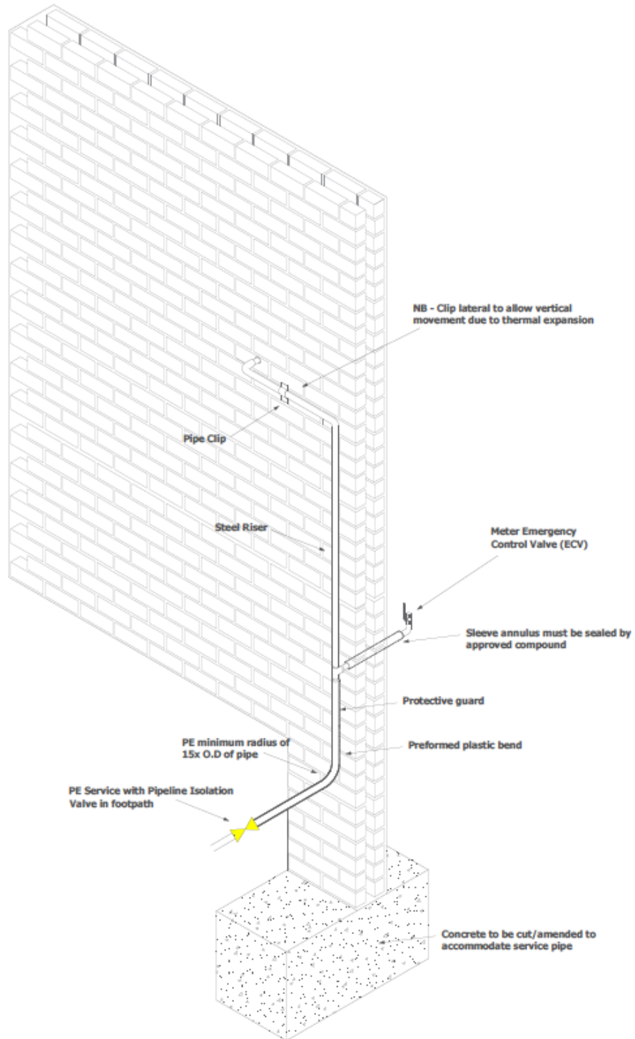
Figure 23 – External risers up to a maximum of 2 floor levels
