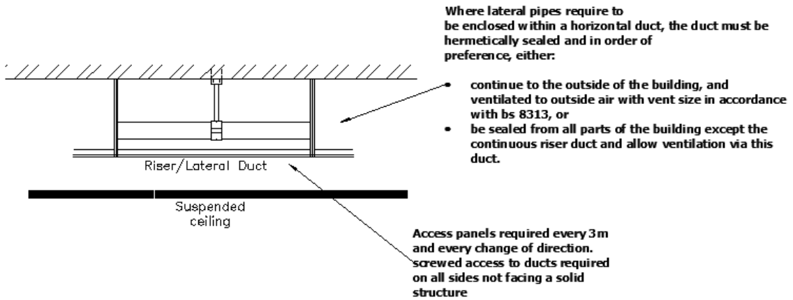
Figure 32 – Ventilation (side elevation)
