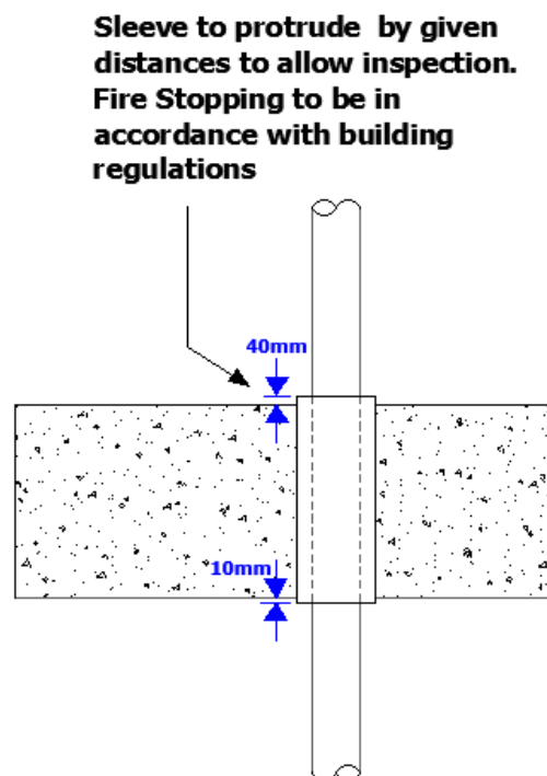
Figure 30 – Sleeves are required to terminate 40mm above floor level and 10mm below so that it is visible for inspection
