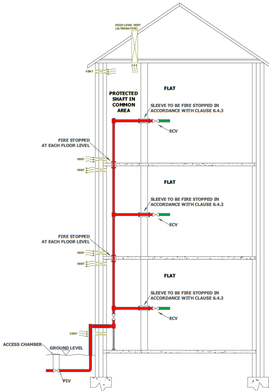
Figure 24 – Internal screwed/welded riser passing through a protective shaft on an outside wall ventilated direct to outside air at each level. Meter locations back on to the riser
