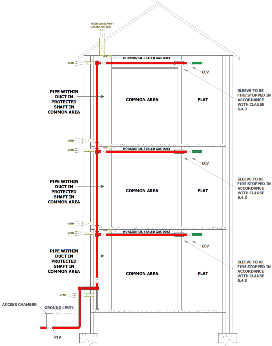
Figure 26 – Internal screwed riser passing through a protective shaft on an outside wall ventilated direct to outside air at each level. Meter locations remote
