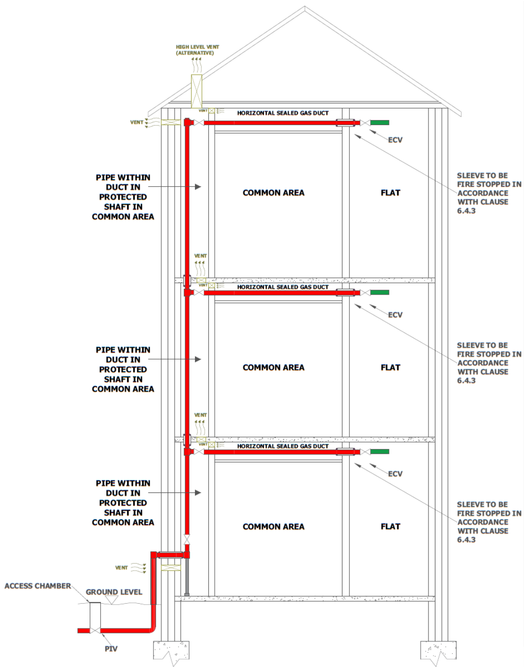
Figure 27 – Internal screwed riser passing through a protective shaft on an outside wall ventilated direct to outside air at the top and bottom of the riser. Meter locations remote
