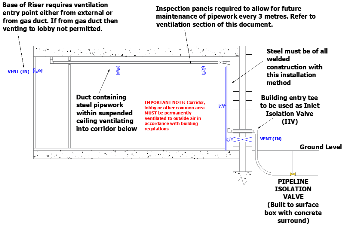
Figure 28 – Internal welded riser with duct indirectly ventilated to outside air via the corridor, lobby, or other common area
