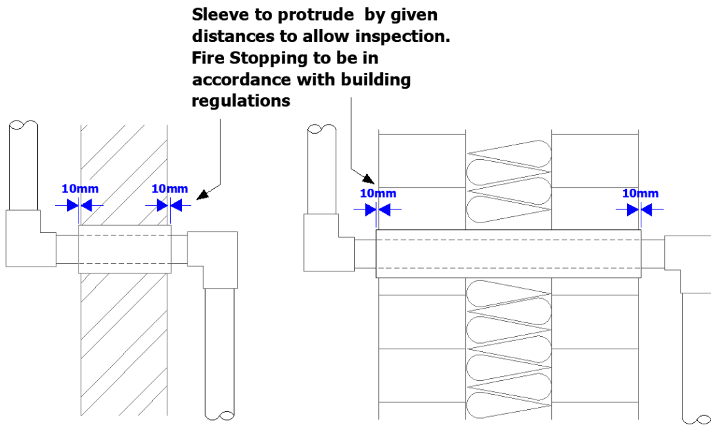
Figure 31 – Fire stopping and sleeving requirements for risers and laterals passing through walls or between fire compartments
