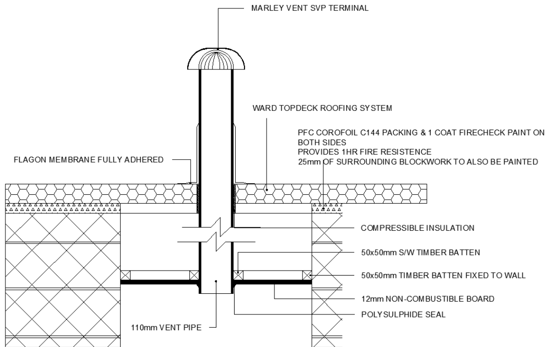
Figure 36 – Example specification if riser shafts are to be ventilated via rooftop ducts. The detail shall be determined by the Developer
