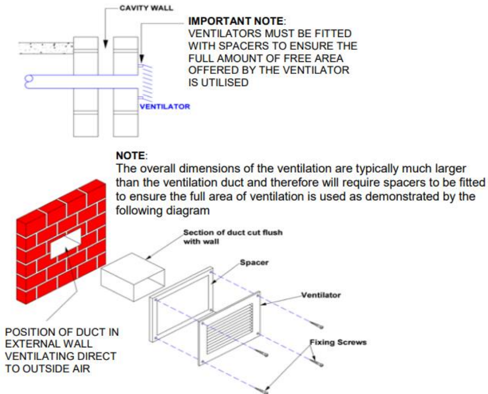
Figure 35 – Spacers must be used to ensure the full free area offered by the vent
