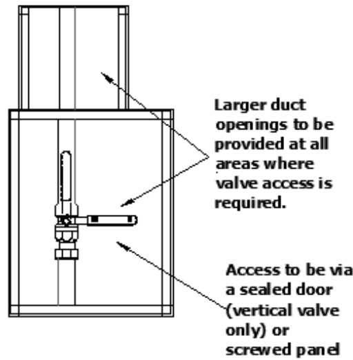
Figure 34 – Vertical valve access (front elevation)
